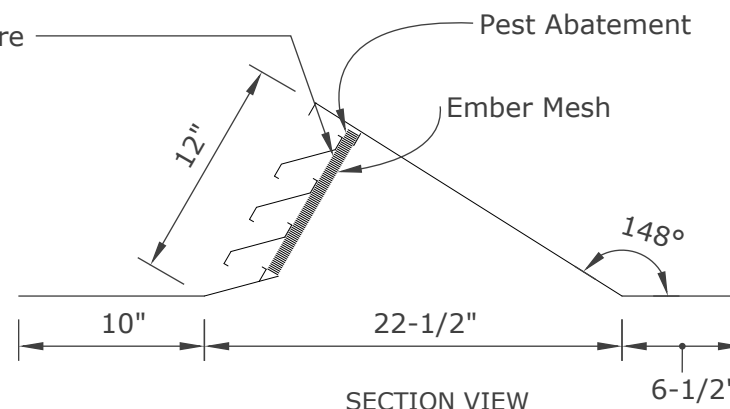
SECTION VIEW
