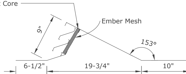
SECTION VIEW
