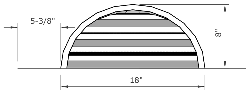
FRONT VIEW
