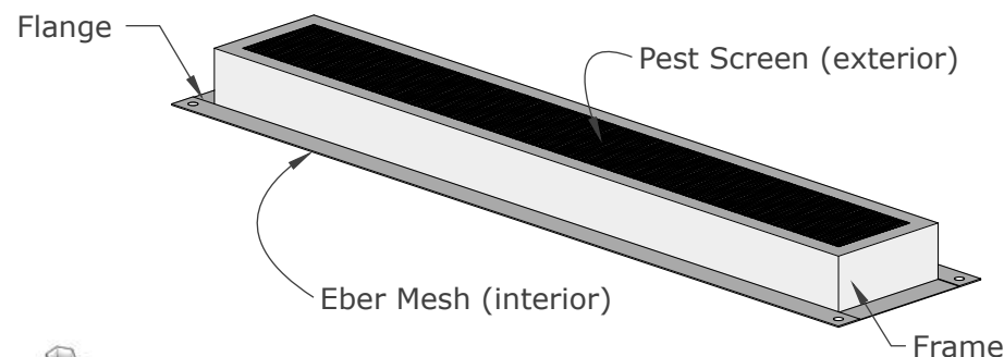
ISOMETRIC VIEW
