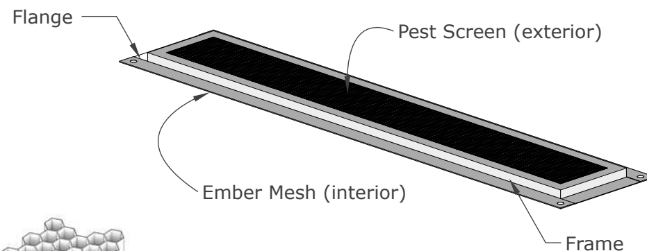
ISOMETRIC VIEW
