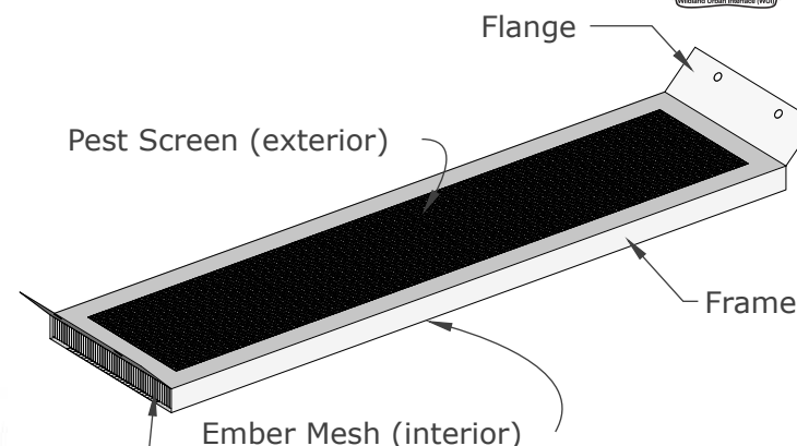
ISOMETRIC VIEW
