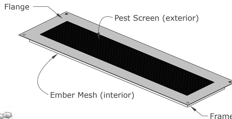
ISOMETRIC VIEW
