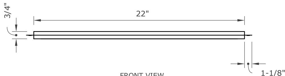
FRONT VIEW
