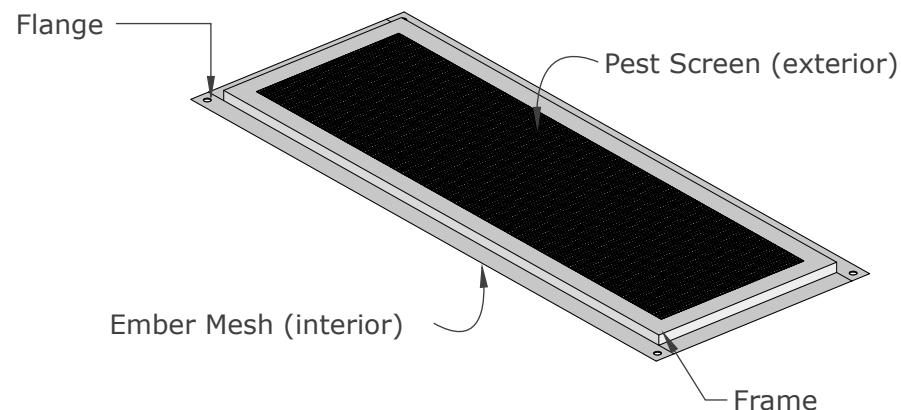
ISOMETRIC VIEW
