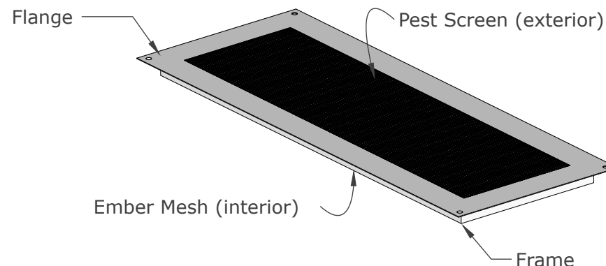
ISOMETRIC VIEW
