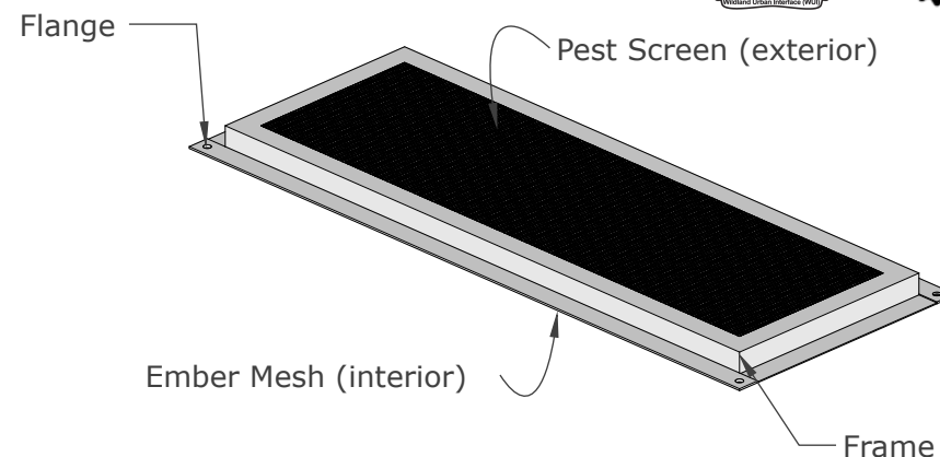
ISOMETRIC VIEW
