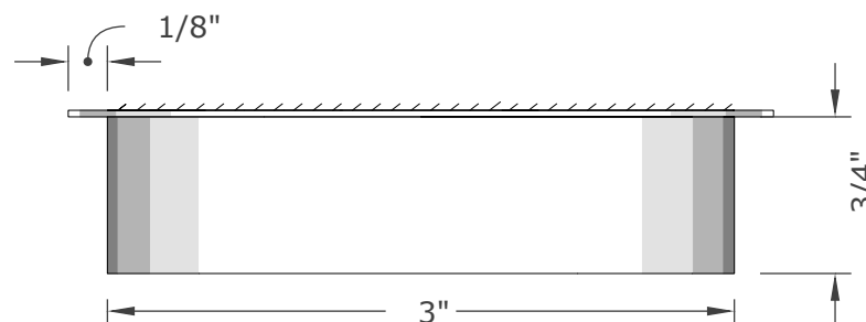
SIDE VIEW
