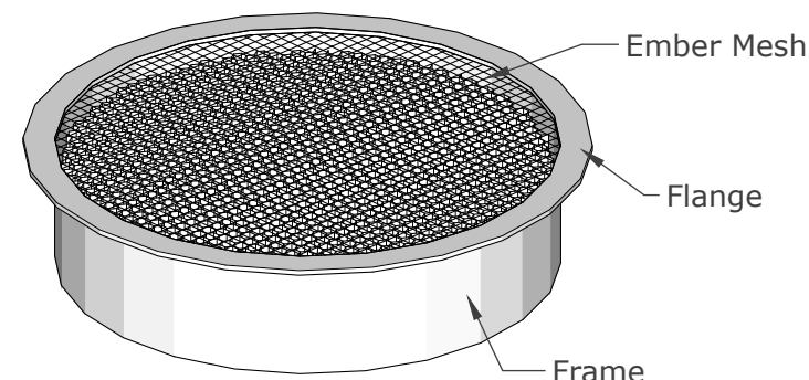
ISOMETRIC VIEWS
