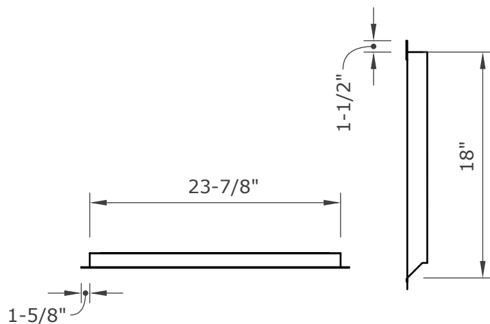
Frame Only - profile views
