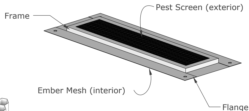
ISOMETRIC VIEW
