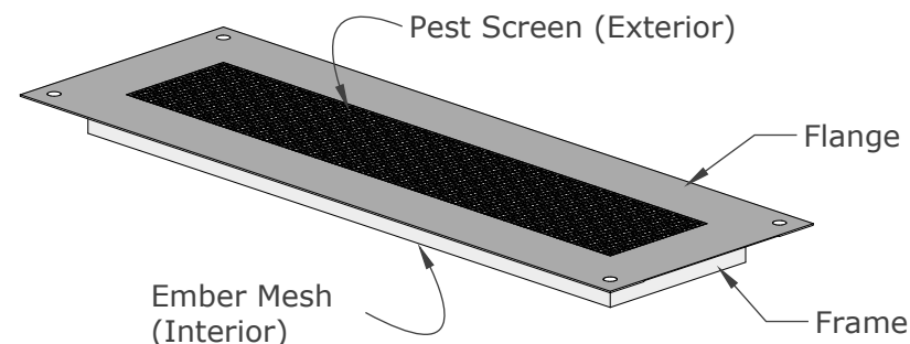
ISOMETRIC VIEW
