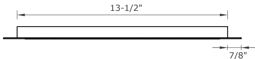
FRONT VIEW
