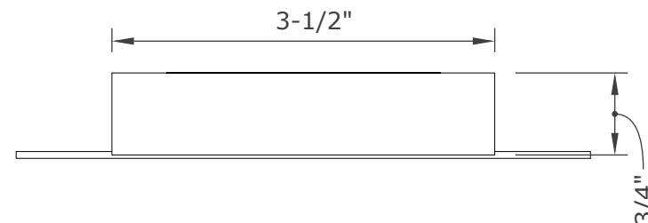
SIDE VIEW
