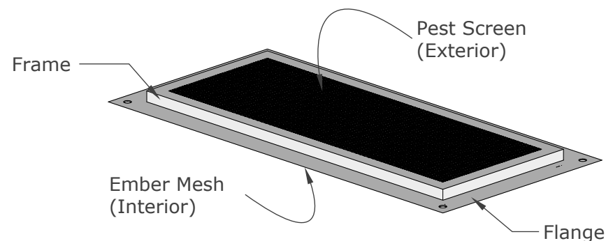
ISOMETRIC VIEW
