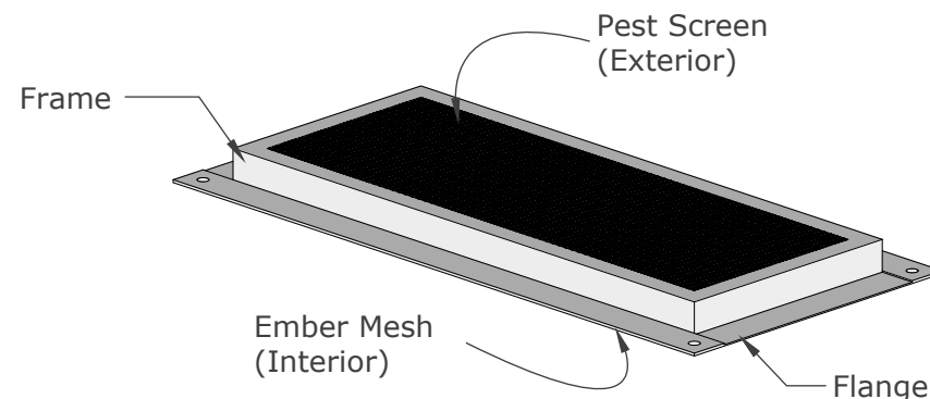
ISOMETRIC VIEW
