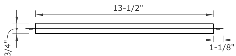
FRONT VIEW
