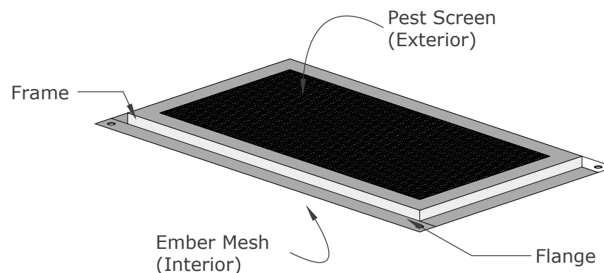
ISOMETRIC VIEW
