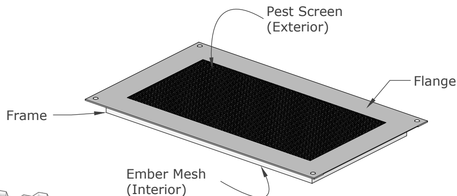
ISOMETRIC VIEW
