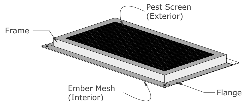
ISOMETRIC VIEW
