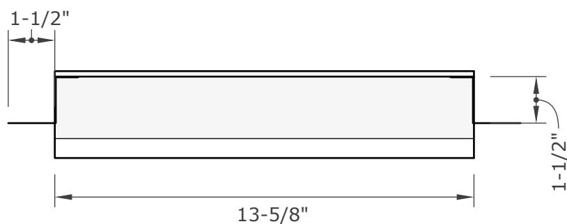
END VIEW
