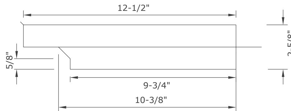
SIDE VIEW
