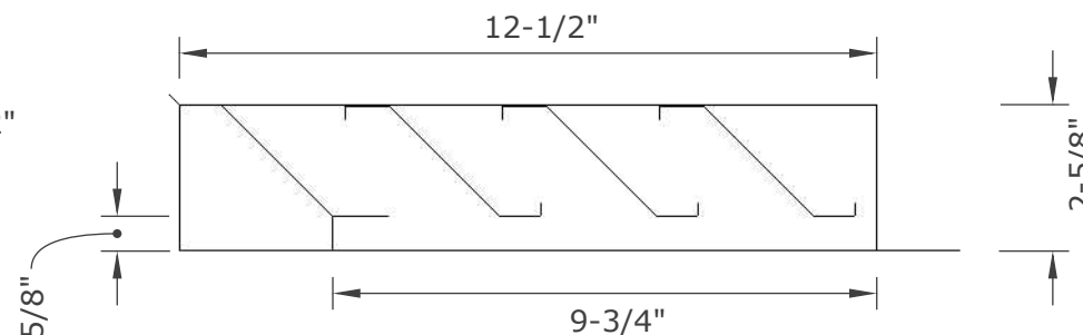
SIDE VIEW
