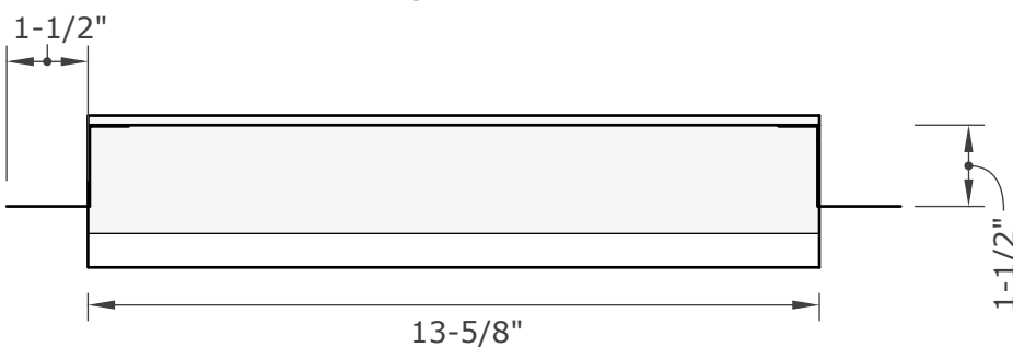
END VIEW
