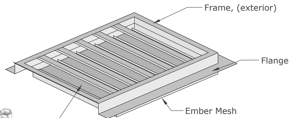
ISOMETRIC VIEW
