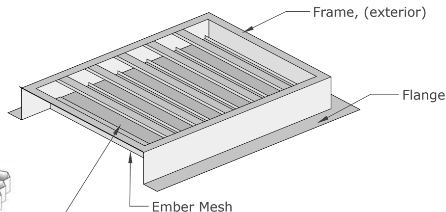
ISOMETRIC VIEW
