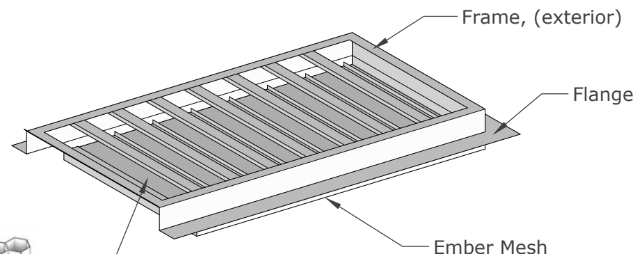
ISOMETRIC VIEW
