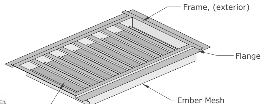
ISOMETRIC VIEW
