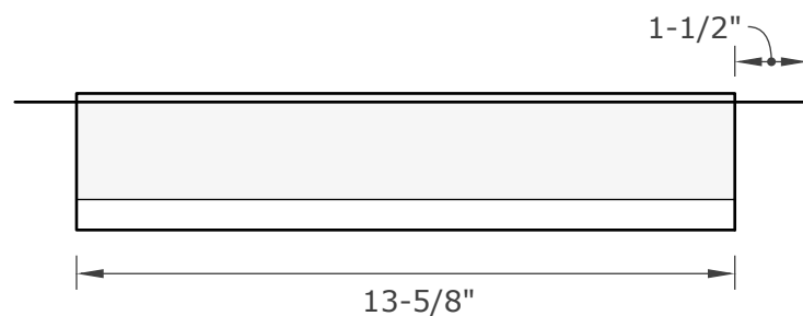
END VIEW
