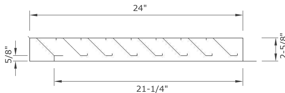
SIDE VIEW
