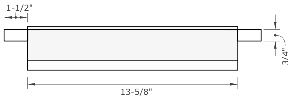
END VIEW
