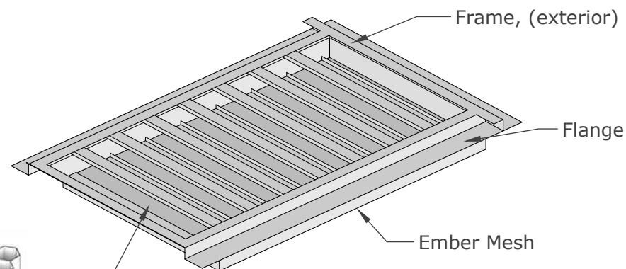
ISOMETRIC VIEW
