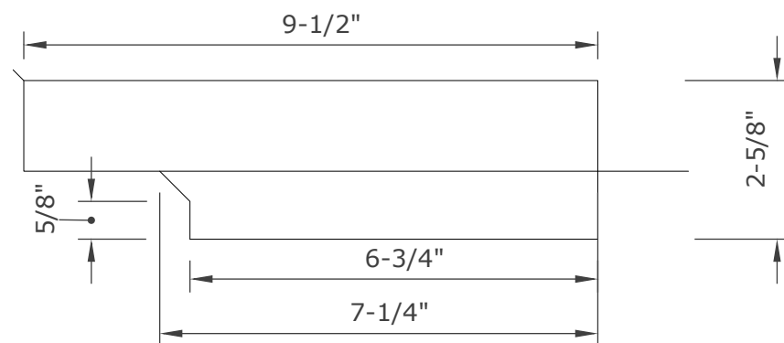
END VIEW
