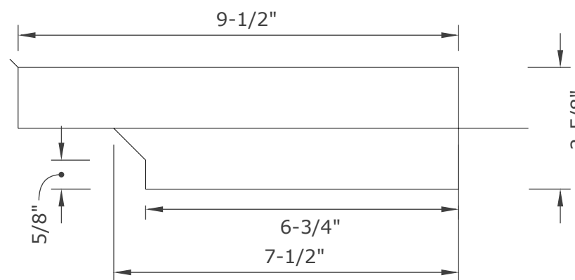
END VIEW
