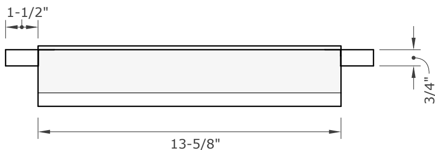
END VIEW
