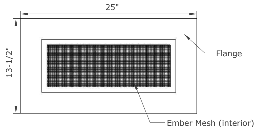
BOTTOM VIEW
