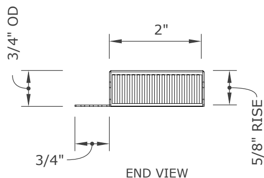
END VIEW
