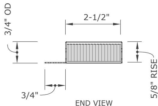
END VIEW
