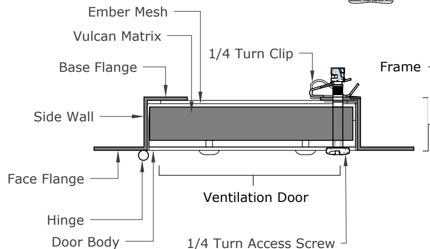
DETAILED VIEW
