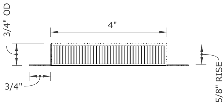
END VIEW
