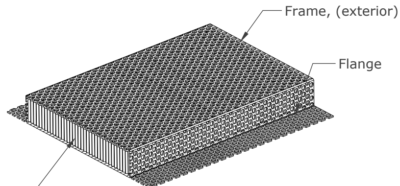
ISOMETRIC VIEWS
