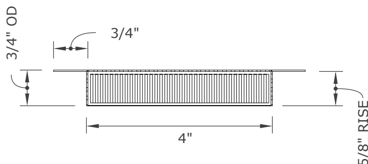
END VIEW
