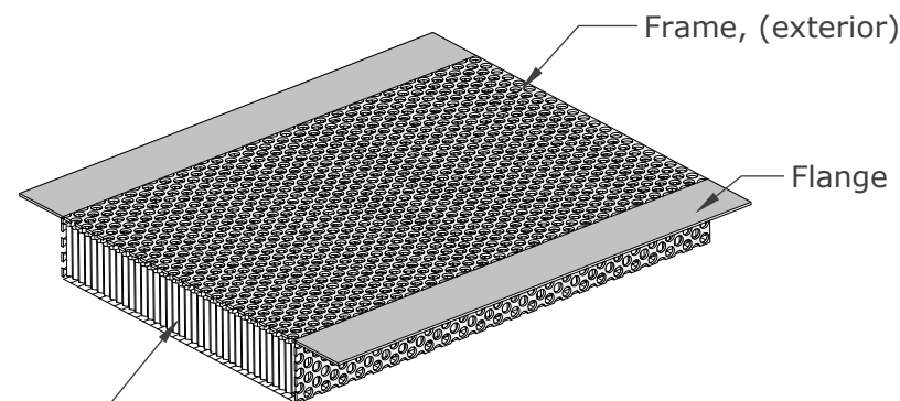
ISOMETRIC VIEWS
