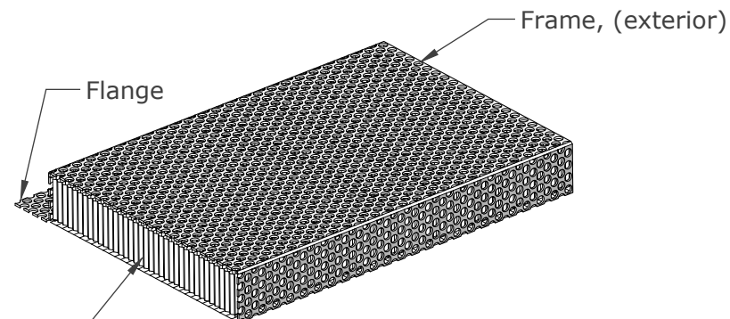
ISOMETRIC VIEWS
