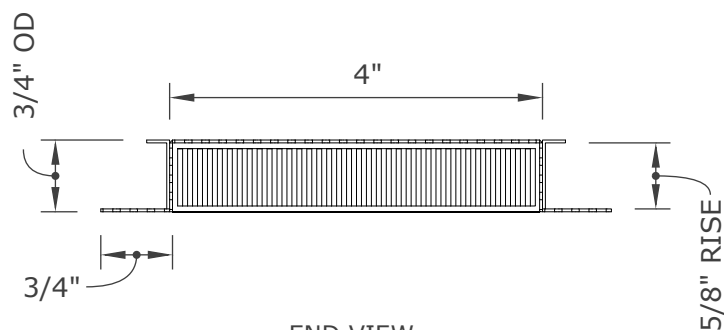
END VIEW
