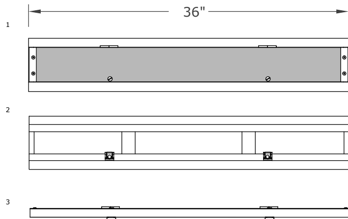
TOP, BOTTOM, ELEVATION VIEWS
