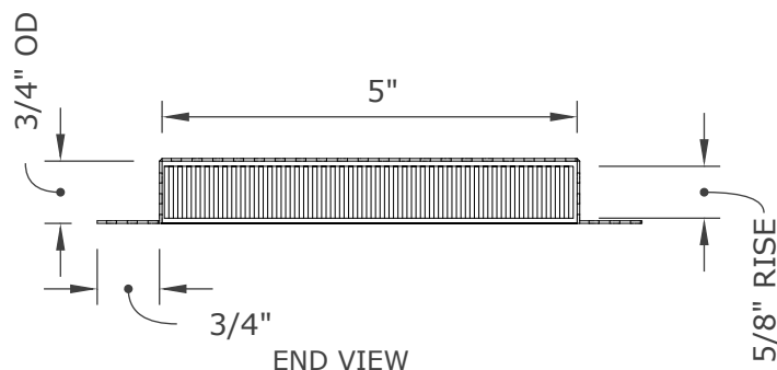
END VIEW
