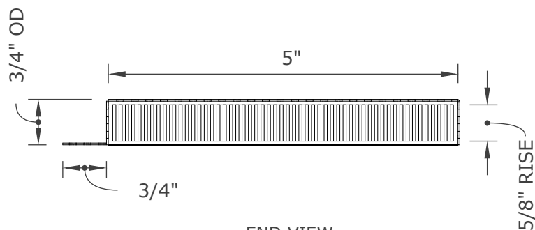
END VIEW
