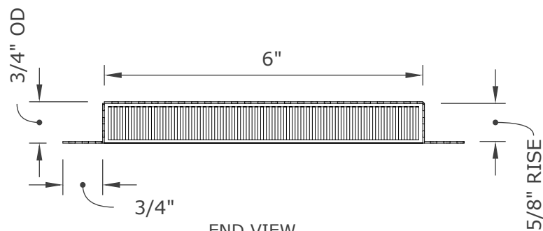
END VIEW
