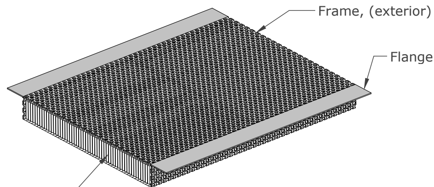
ISOMETRIC VIEWS
