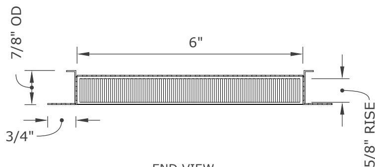
END VIEW
