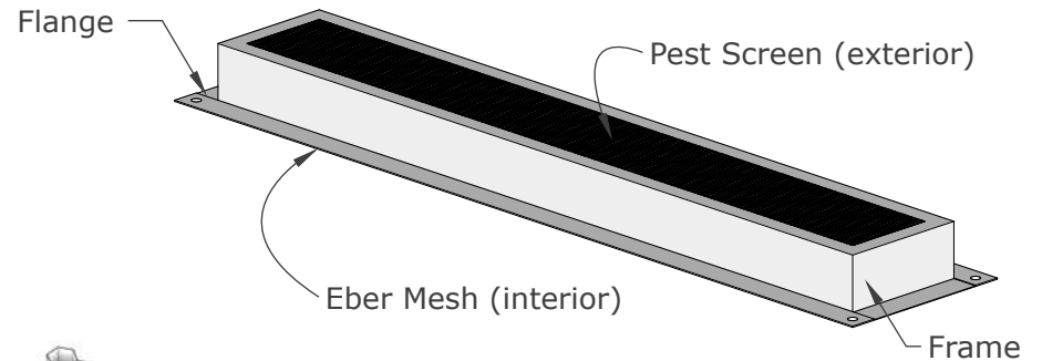
ISOMETRIC VIEW
