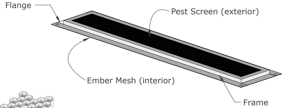
ISOMETRIC VIEW
